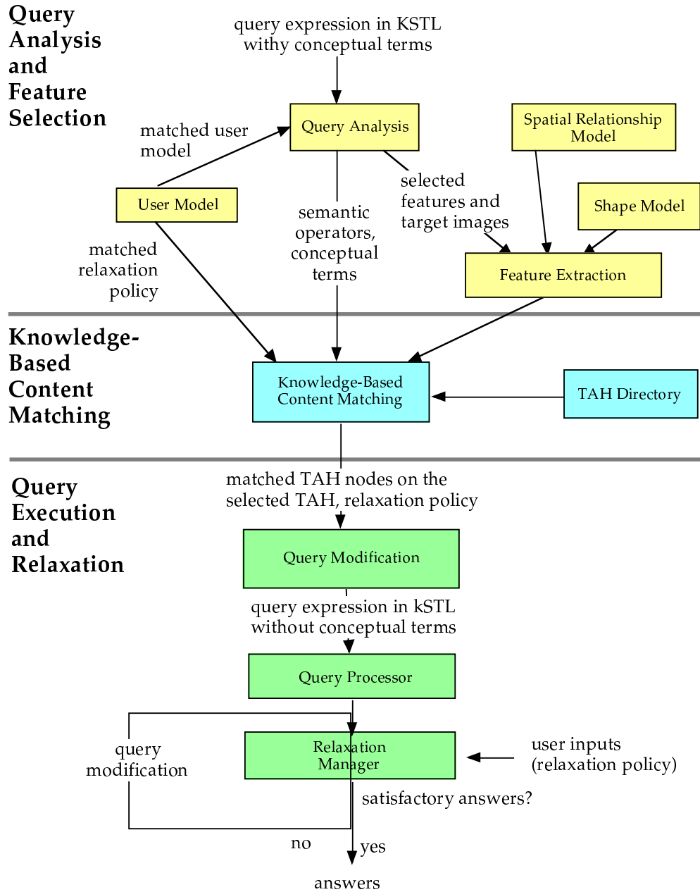
Figure 13: The flow diagram of knowledge-based query processing.
