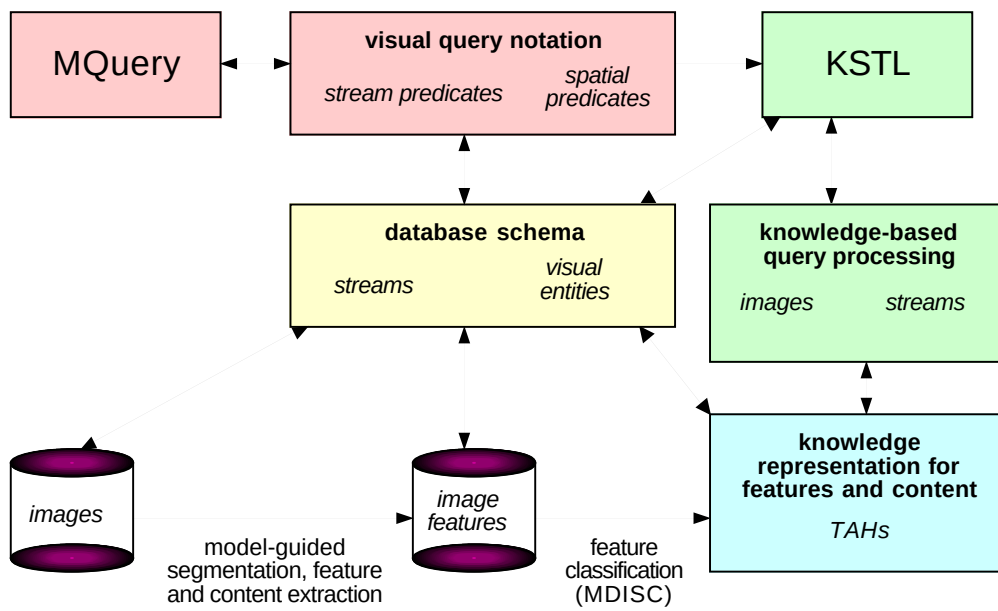
Figure 14: Data flow and system architecture.
