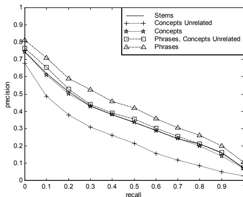
Figure 1. Comparison of the average precision-recall over 105 queries.
